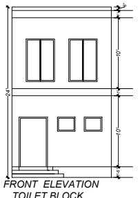
FRONT ELEVATION TOILET BLOCK
