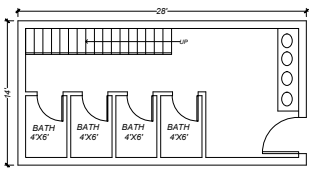
GROUND FLOOR PLAN TOILET BLOCK
