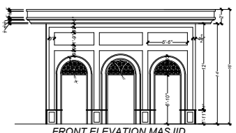
FRONT ELEVATION MASJID
